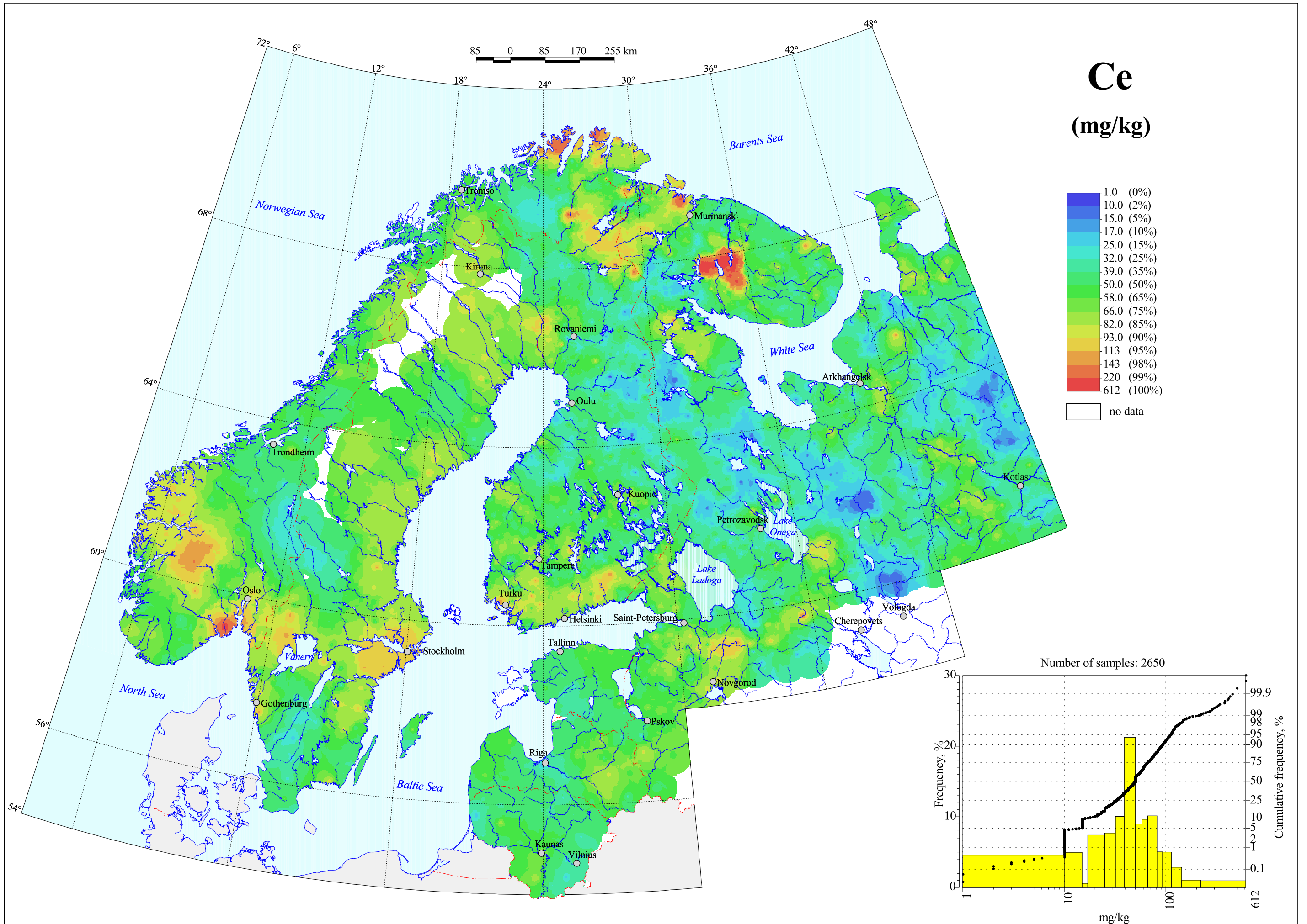
Cerium in C-horizon, Grain Size <2 mm, Total Content
